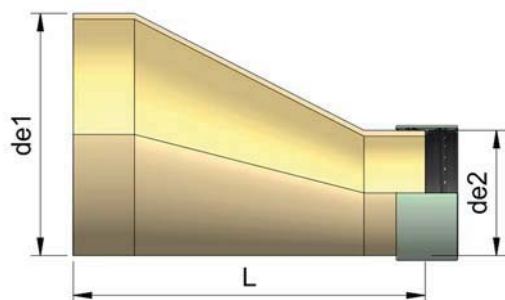
Lengths for concentric and eccentric reducers
