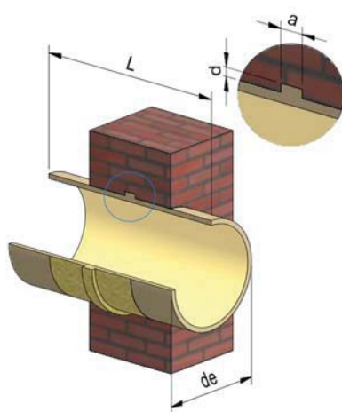
Structural adapter, sand covered with thrust ring (TYPE F)
