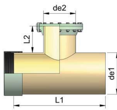
Inspection pieces
