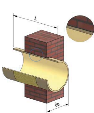
Structural adapter, sand covered (TYPE E)
